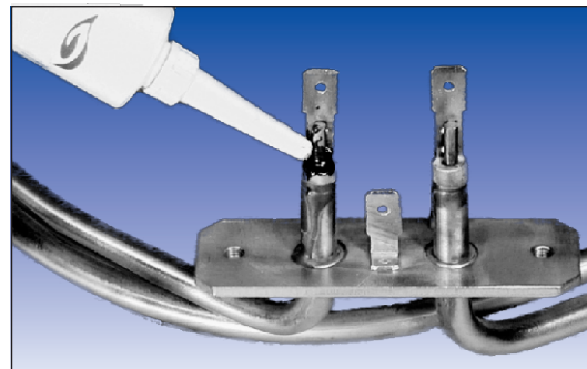
4700 Seals Electrical Feed Thrus for a High Temperature Heater
